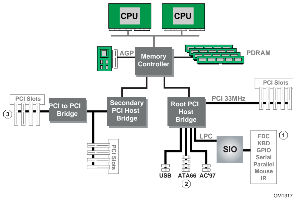
Figure 135. Example Computer System
