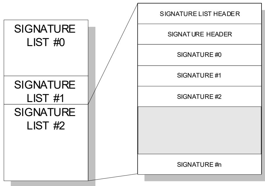
Figure 78. Signature lists
