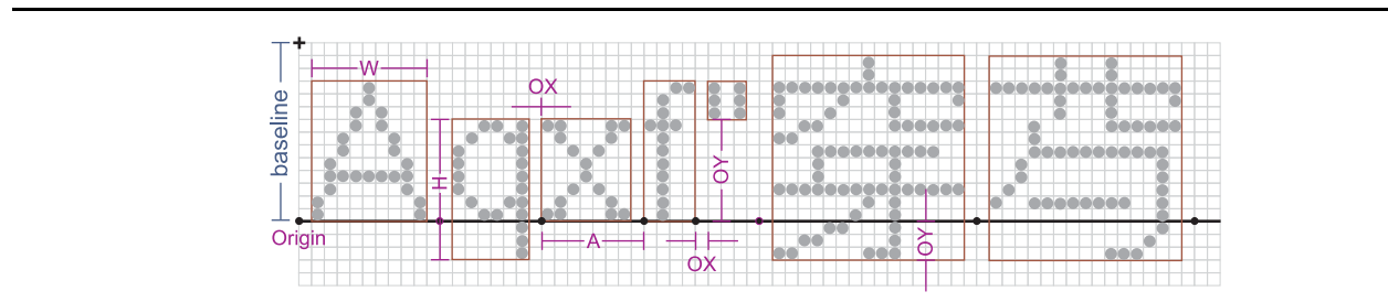
Figure 102. Aligning Glyphs
