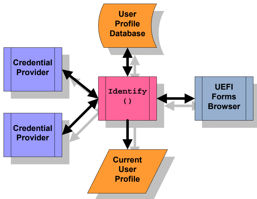
Figure 133. User Identity
