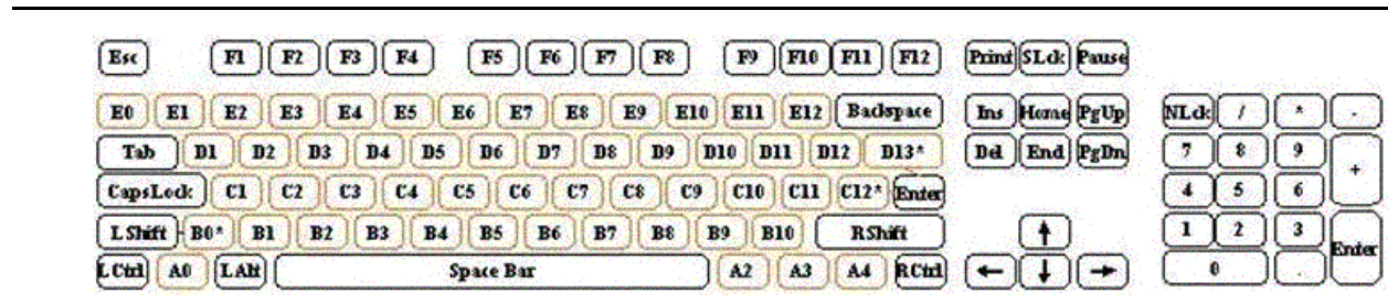
Figure 91. Keyboard Layout
