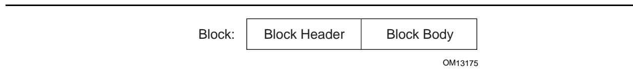
Figure 58. Block Structure
