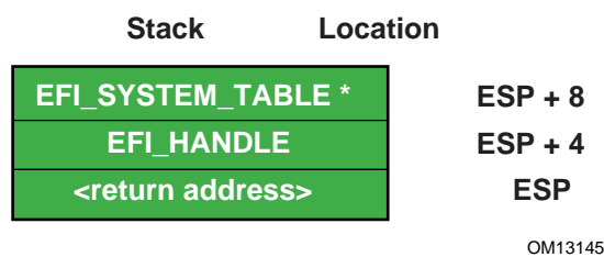
Figure 3. Stack after AddressOfEntryPoint Called, IA- 32
