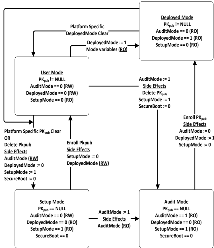
Figure 77. Secure Boot Modes
