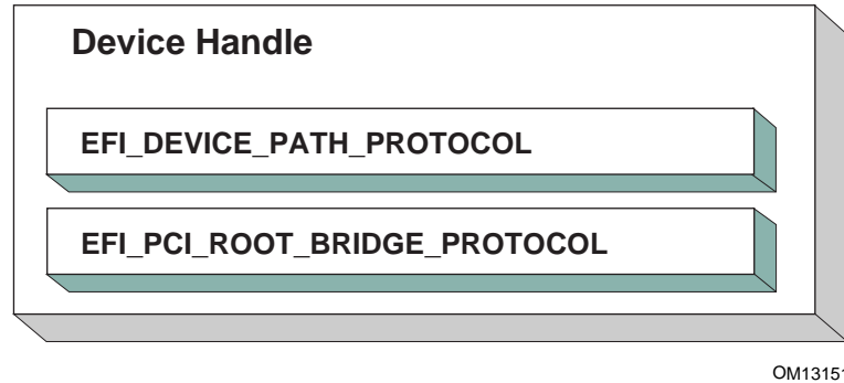
Figure 11. PCI Root Bridge Device Handle
