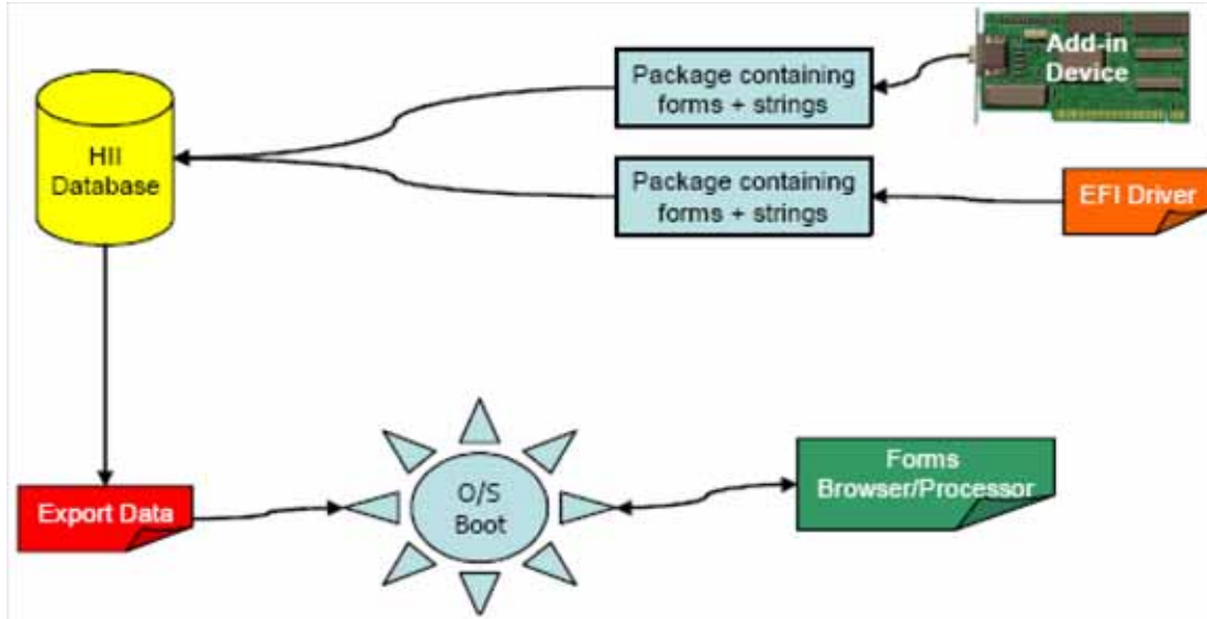
Figure 89. O/S-Present Forms Browser/Processor
