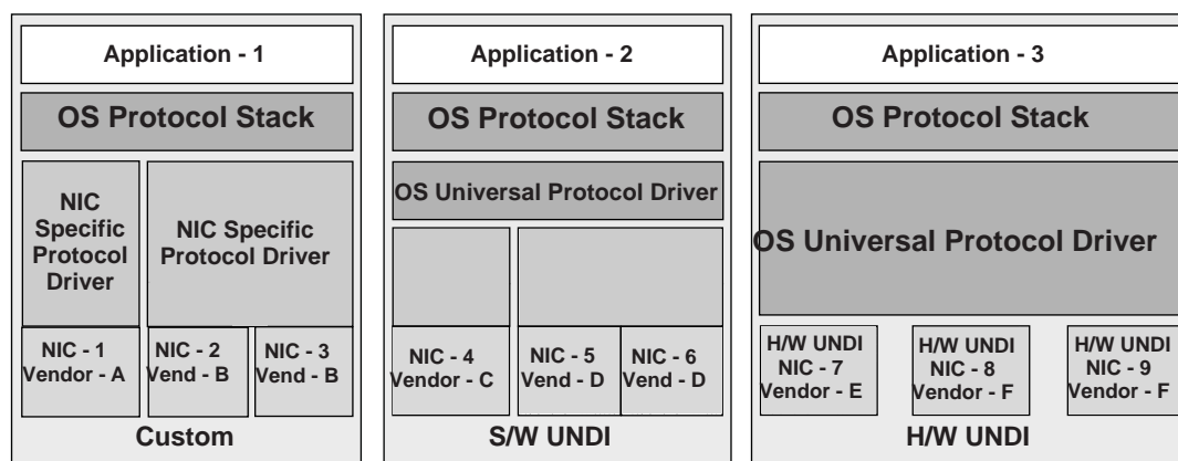
Figure 138. Network Stacks with Three Classes of Drivers
