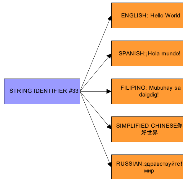
Figure 96. String Identifiers
