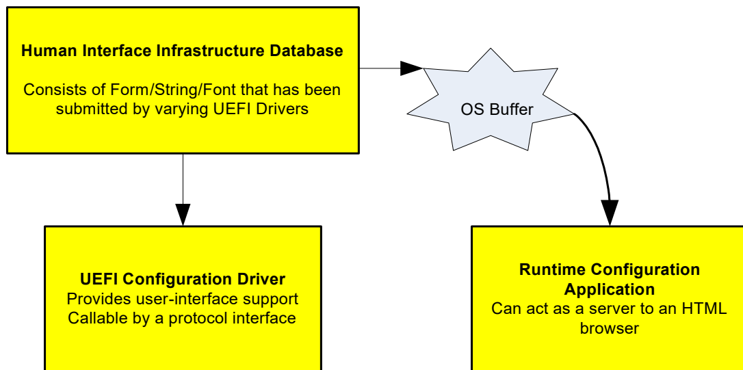
Figure 106. OS Runtime Utilization
