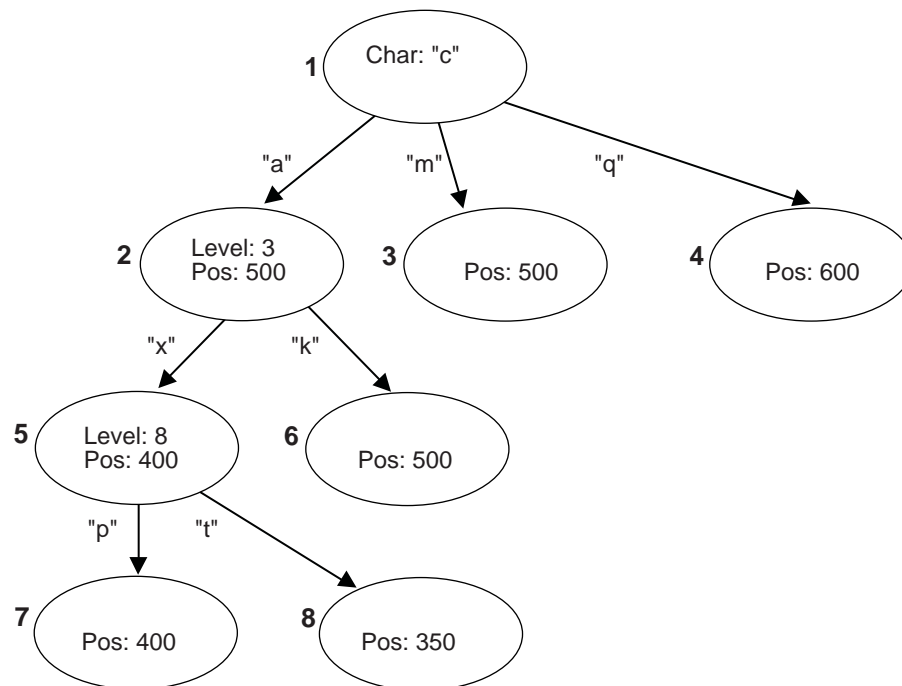
Figure 60. String Info Log Search Tree
