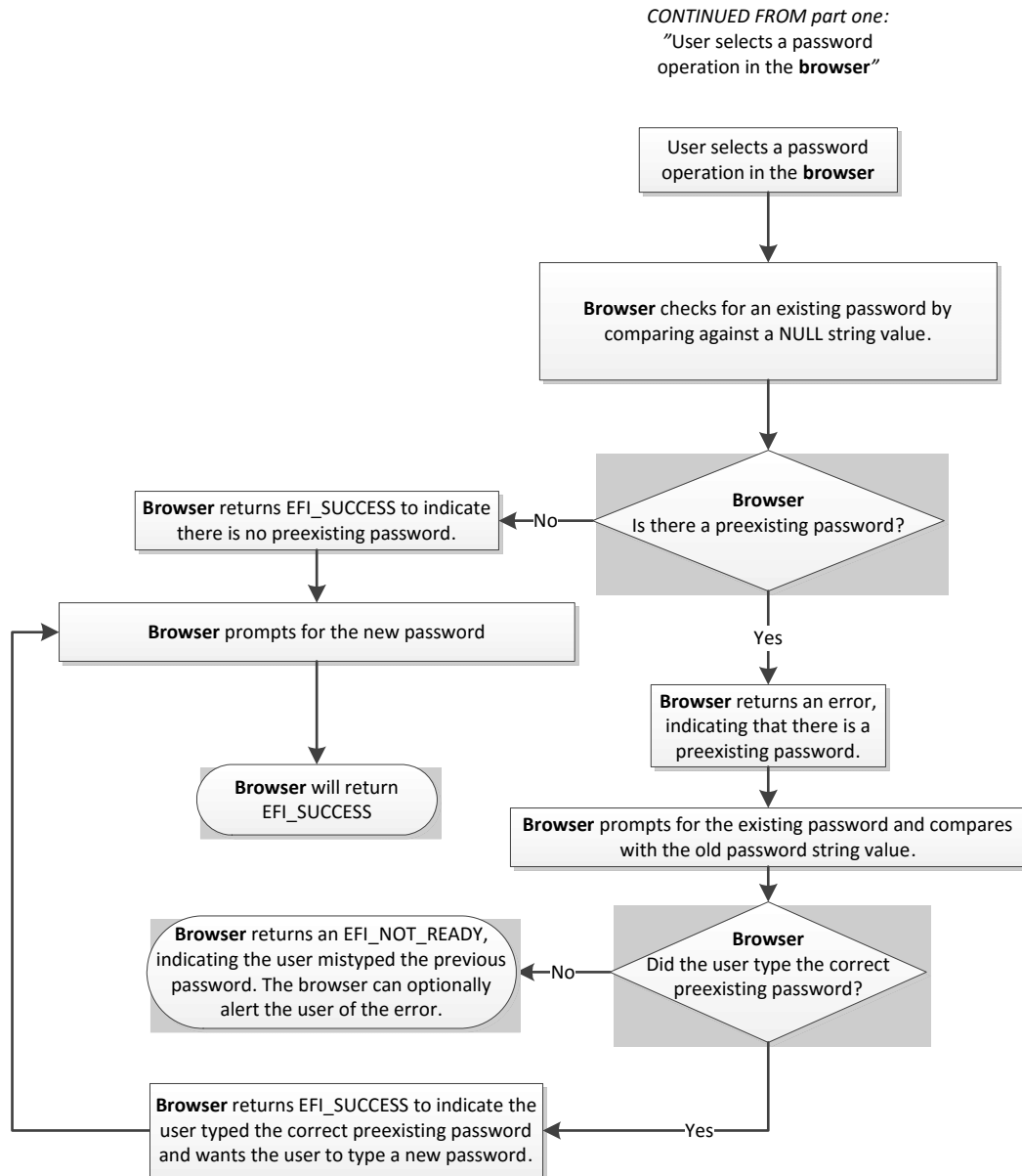
Figure 128. Password Flowchart (part two)
